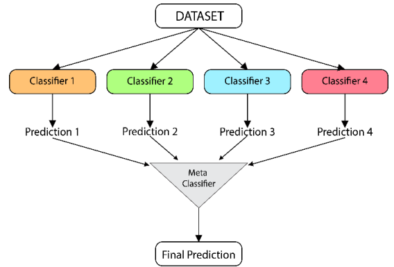
Fig. 5. Representation of Stacking Classifier
